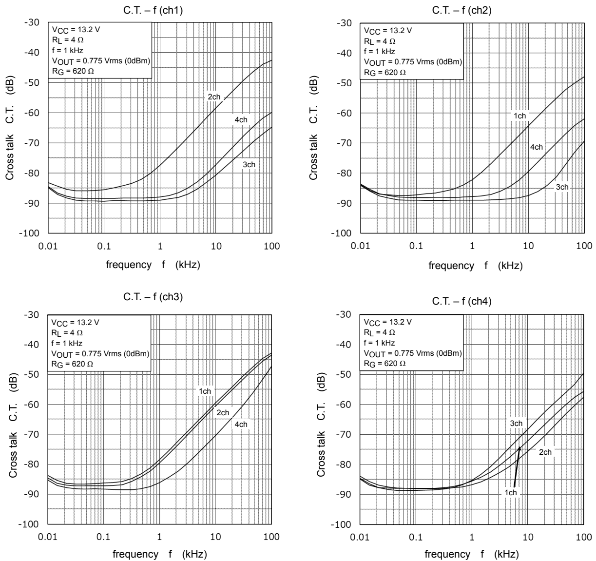
Fig. 11-6 Frequency Characteristics of Cross Talk
