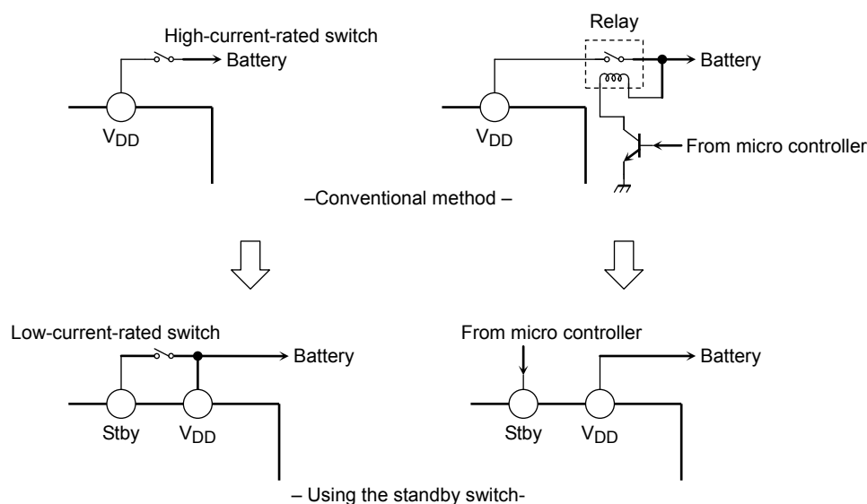
Figure 2 Standby switch
