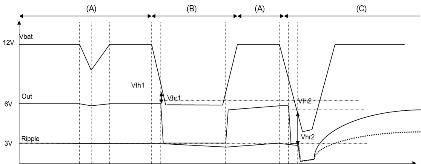
Figure 9 Output VDD/2 voltage in lowering VDD
